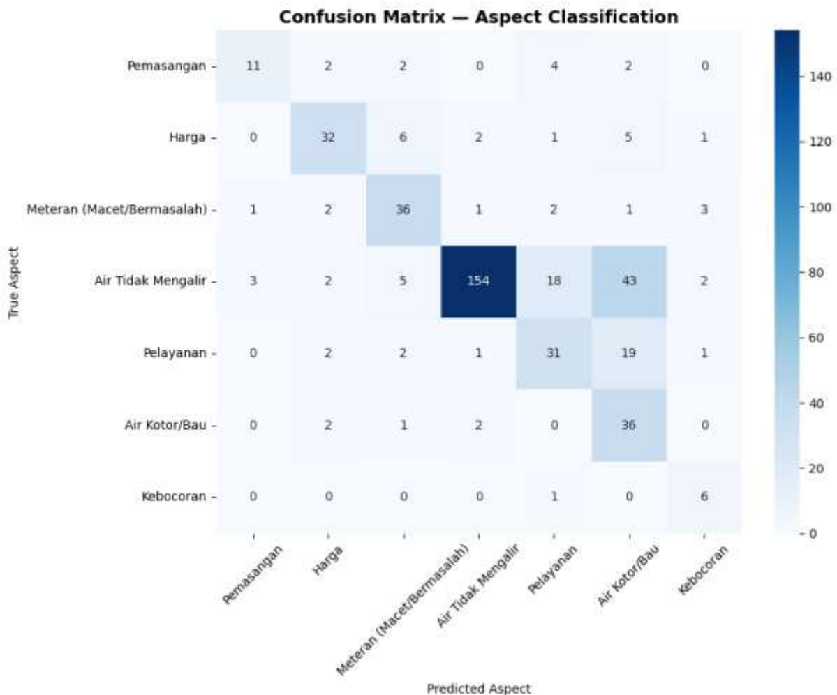
Gambar 4. 3. Confusion Matrix Skenario 3
